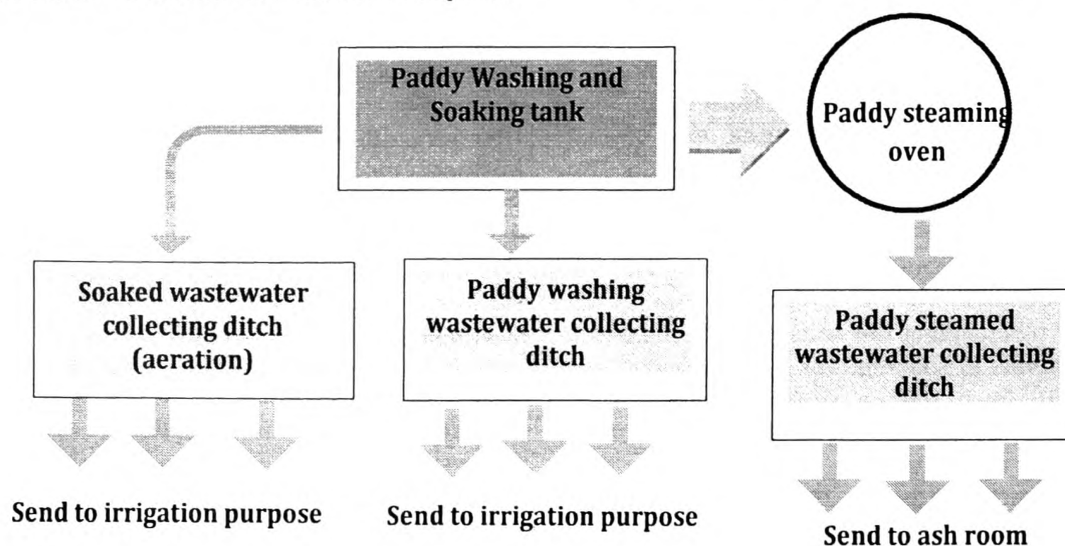
Figure 1: Modified wastewater discharge system
