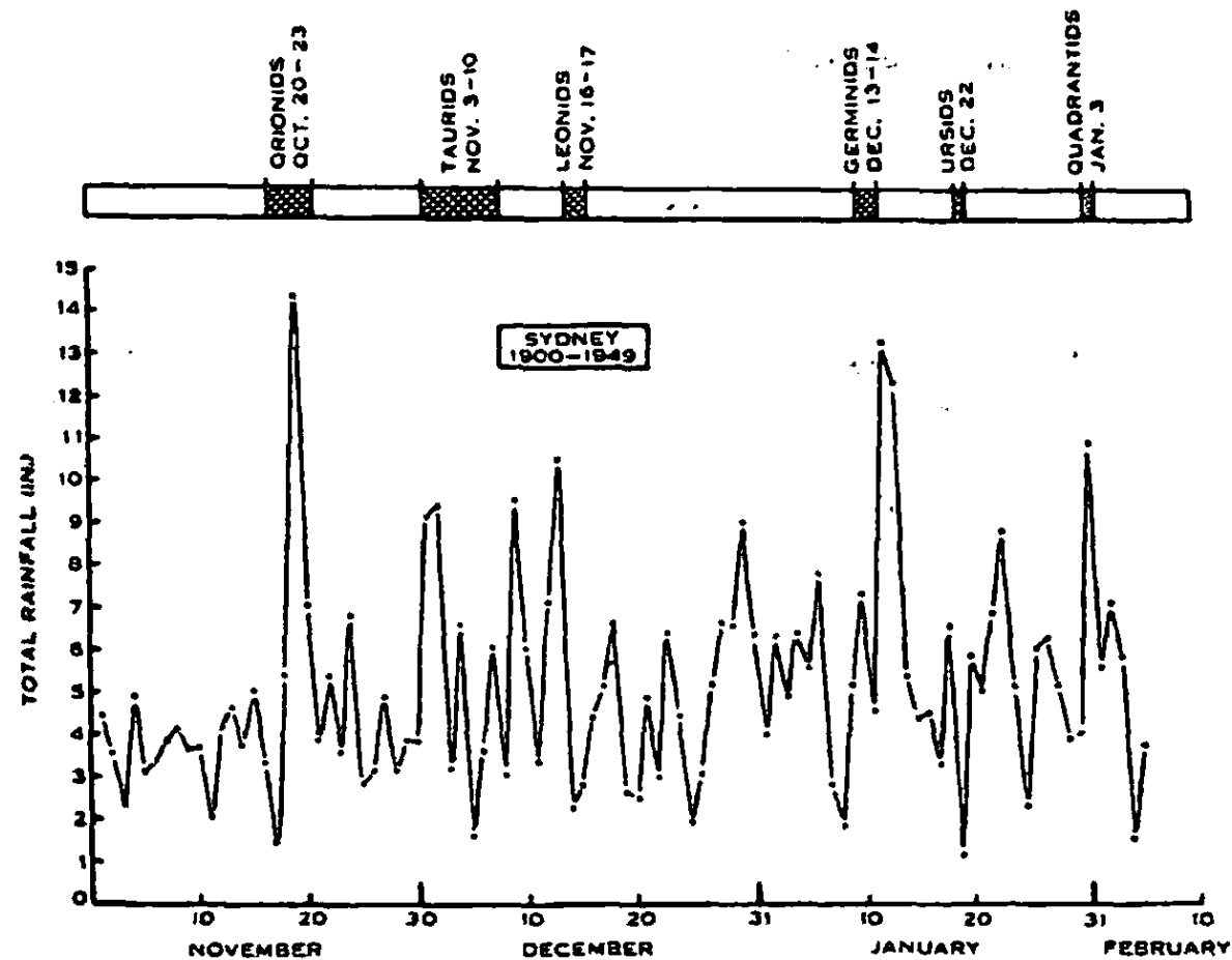
Fig. 4.—Daily rainfall of Sydney for November, December, and January for the period 1900–1949, together with dates of the main meteor streams displaced 29 days in time.
