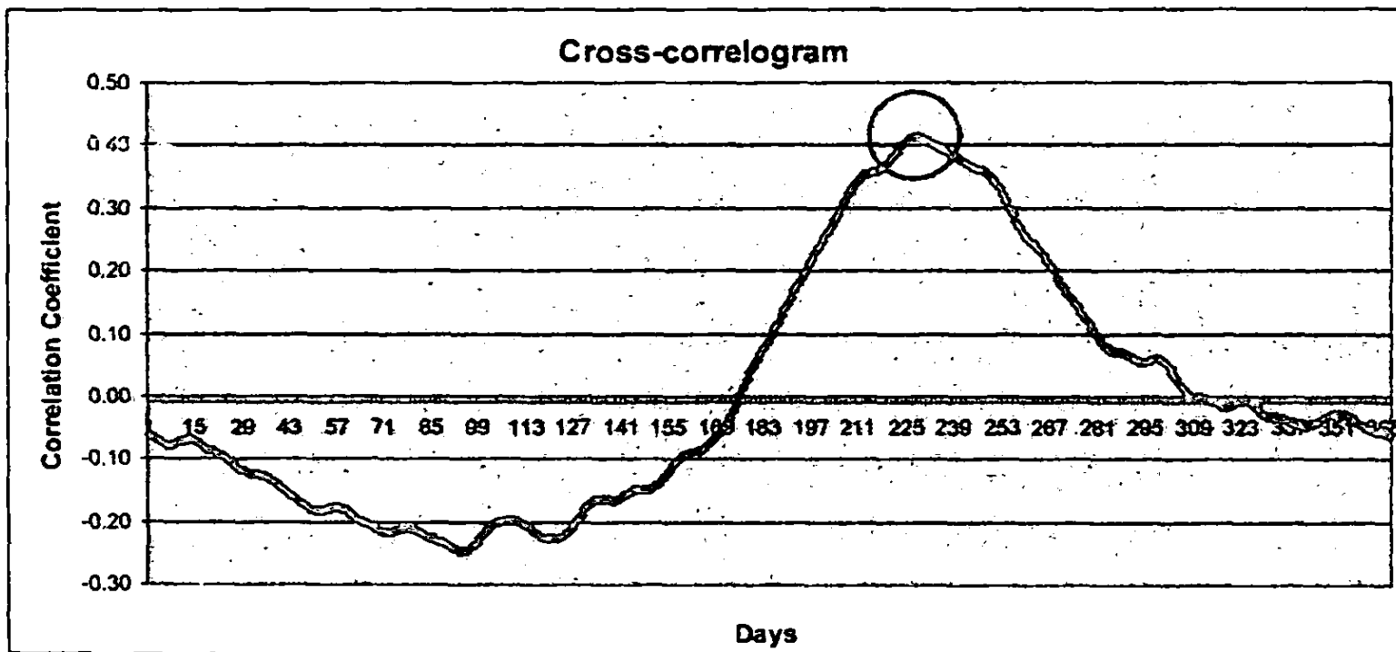
Figure 4: The cross-correlogram - correlation coefficients against the time lag to interpret the set of autocorrelation coefficients as a result of cross-correlation test for 365 days. The absolute maximum being on 226 days time lag
