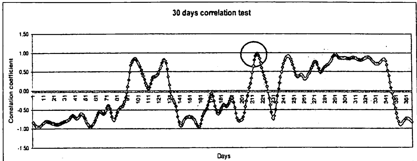
Figure 5: The correlogram of 30 days correlation test for meteor series Jul 09 to Aug 08, indicates highest correlation 0.97 after 216 days of meteor activity.
