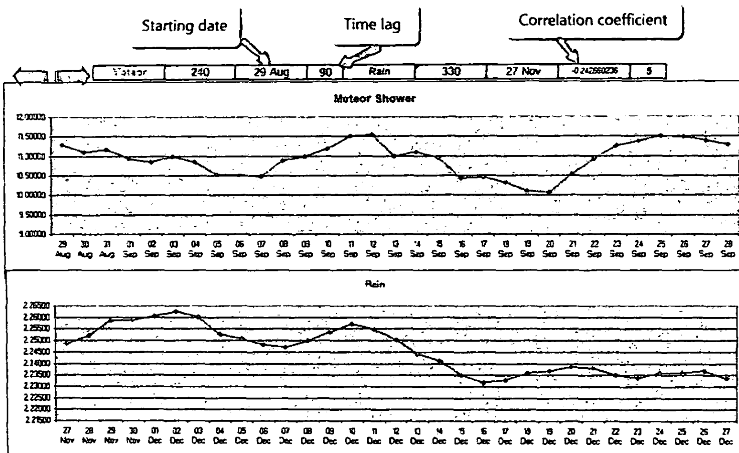
Figure 2: An interface of comparing meteor series and precipitation series. Using this graphical software, relationship and graphical form of two series for any time lag can be illustrated.
