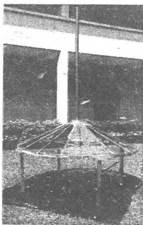
Figure 4: (a) The model chimney dryer in open air (b) Variation of air flow speed (under the collector: x- Natural flow with grass O- covered by black polythene (■) Variation of the environmental wind speed.
