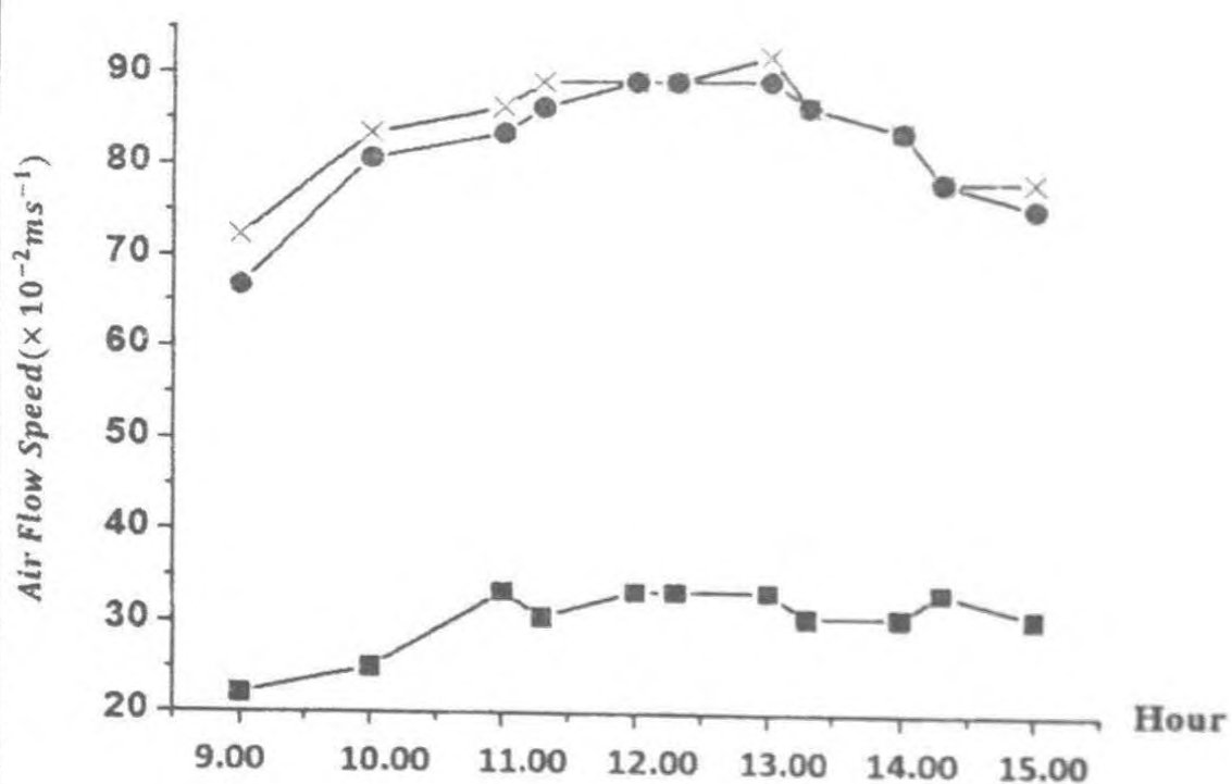
Figure 4: (a) The model chimney dryer in open air (b) Variation of air flow speed (under the collector: x- Natural flow with grass O- covered by black polythene (■) Variation of the environmental wind speed.
