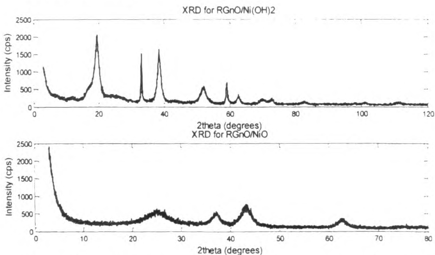
Figure 2: The X-Ray diffraction pattern corresponding to \text{rGO/Ni(OH)}_2 and \text{rGO/NiO} composites
