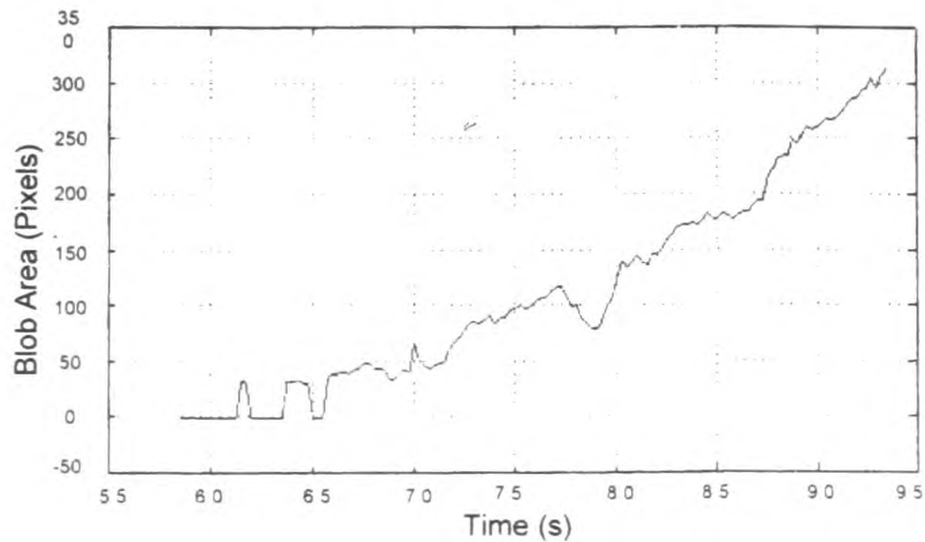
Figure 4: Increasing blob area with time for a non-moving object which may cause a collision.
