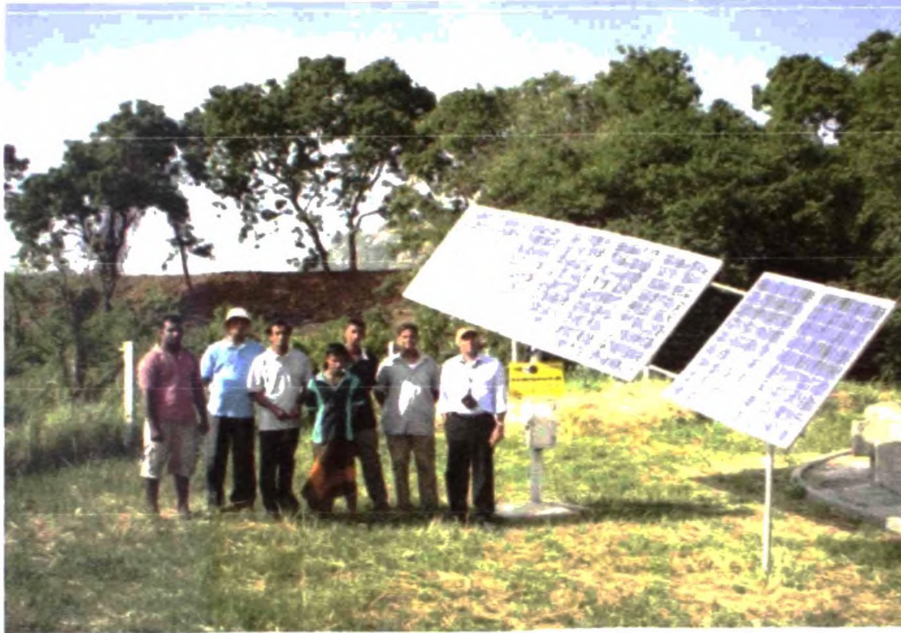
Figure 7: The pilot Solar Village started in 2008 by replacing a diesel water pump by a solar water pumping system.
