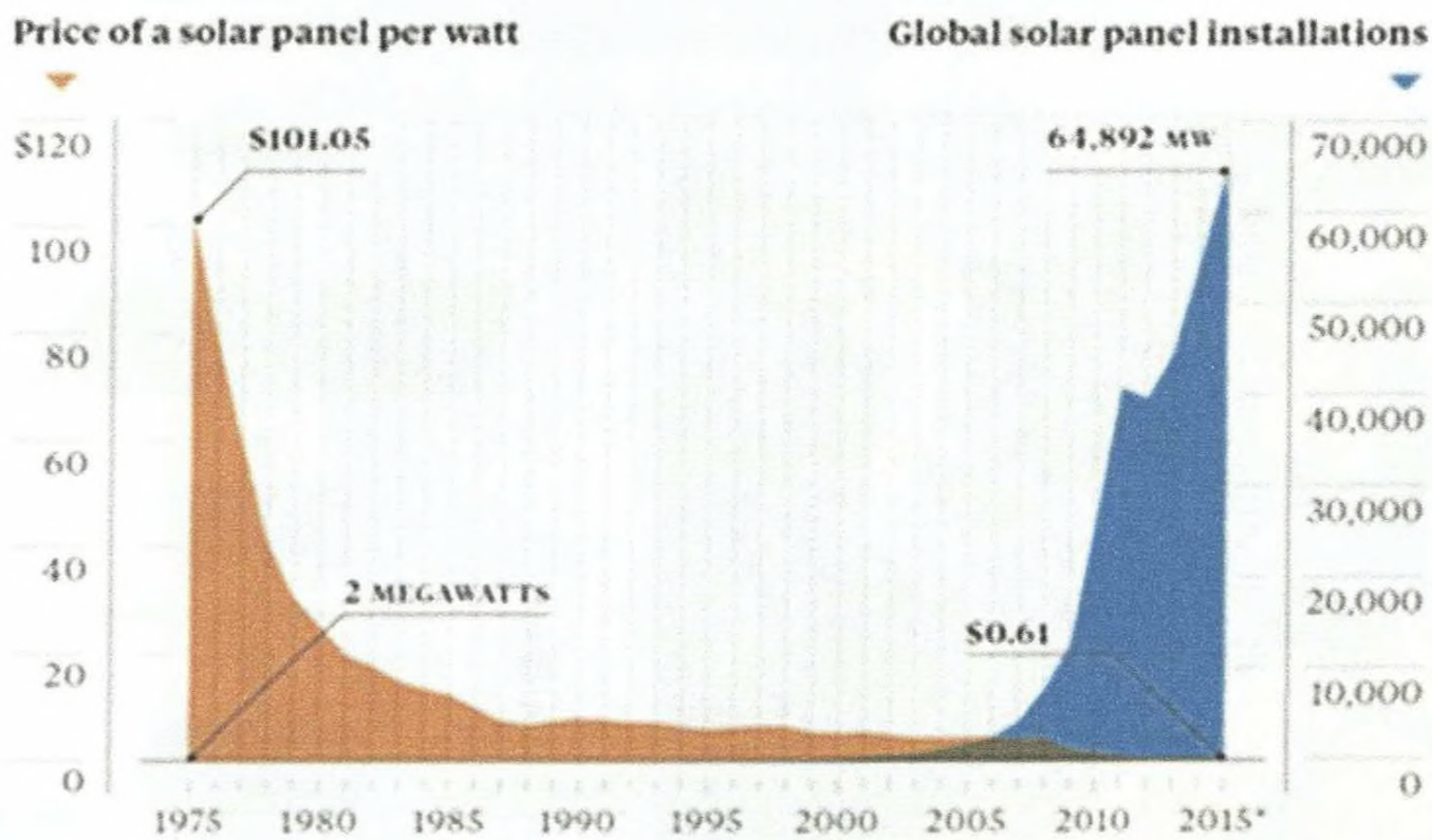
Figure 1: Change of solar panel cost and Global solar panel installations as a function of time. Note the drastic cost reduction and exponential increase in solar energy application between the 1980's and at present.
