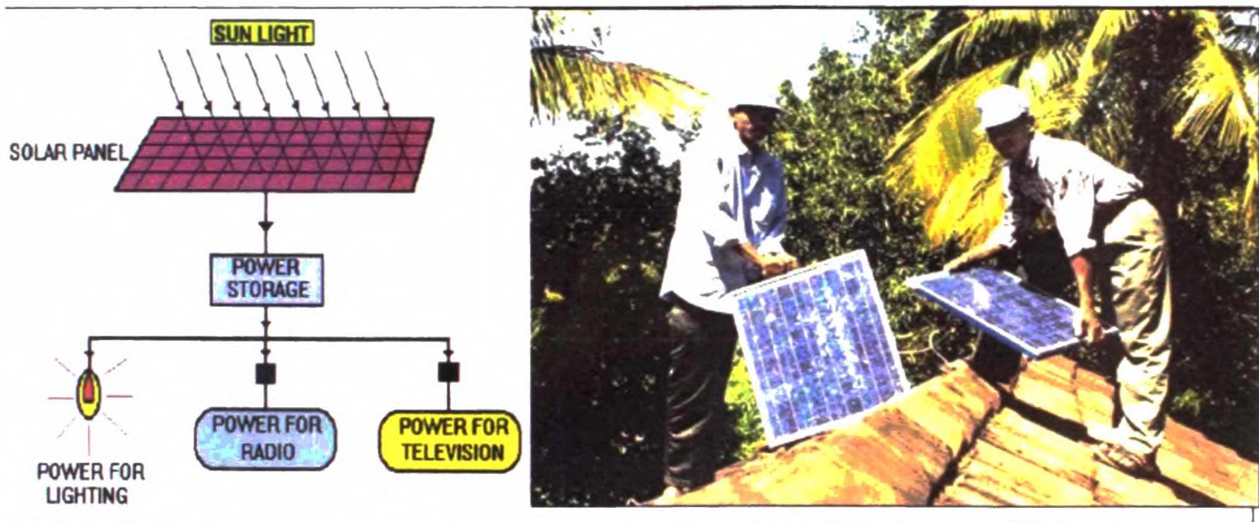
Figure 2: Schematic diagram of a Solar Home System and an example of a real system in Sri Lanka.
