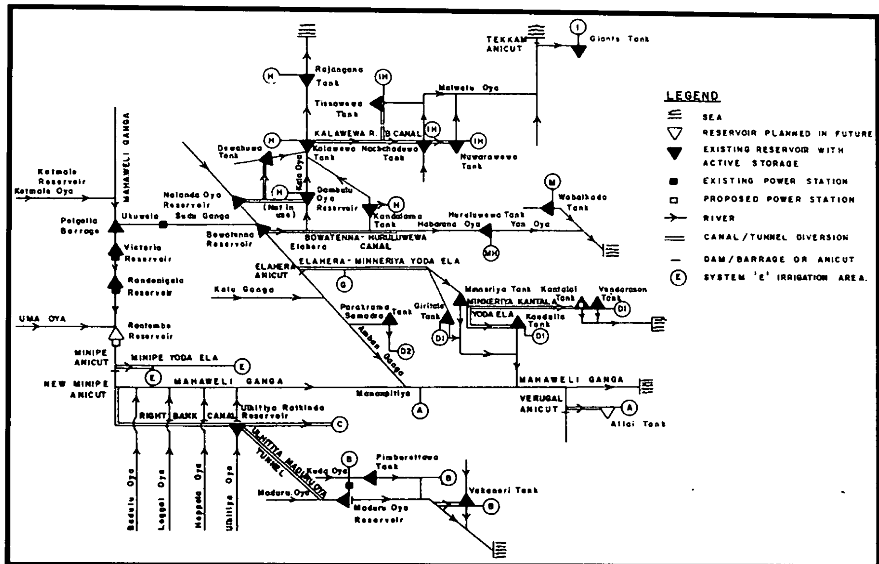
Fig. 4 Water conveyance system of the Mahaweli diversion scheme, illustrating the role of River Mahaweli upper catchment in the upcountry wet zone and eventual dispersal of Mahaweli waters throughout NCP
