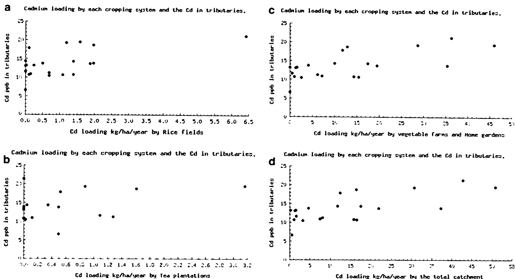
Fig. 5 a Scatter plots of cadmium content in tributary ( \mu\text{g/l} ) and cadmium loading from rice fields in the respective catchment ( \text{kg Cd/ha/year} ). Rank correlation coefficient Kendalls \tau=0.339 and two-sided p=0.038 . b A scatter plot of cadmium content in tributary in ( \mu\text{g/l} ) and cadmium loading from Tea plantations in the respective catchment as ( \text{kg Cd/ha/year} ). Rank correlation coefficient Kendalls \tau=0.441 and two sided p=0.043 . c A scatter plot of cadmium content in tributary in ( \mu\text{g/l} ) and cadmium loading from vegetable
