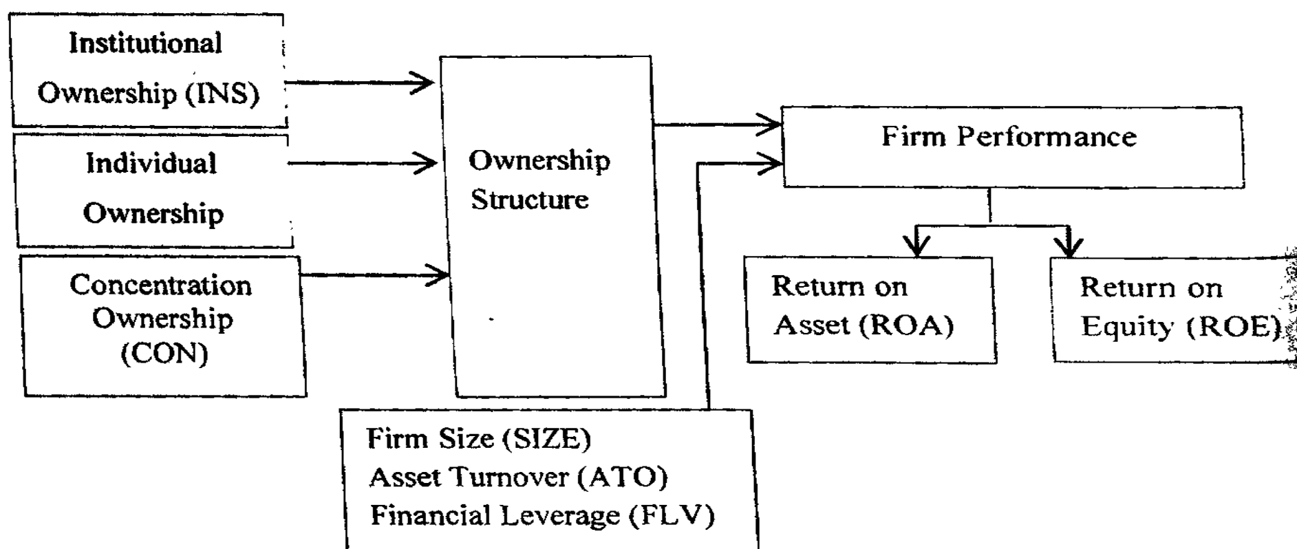
Figure 1: Conceptual Framework
