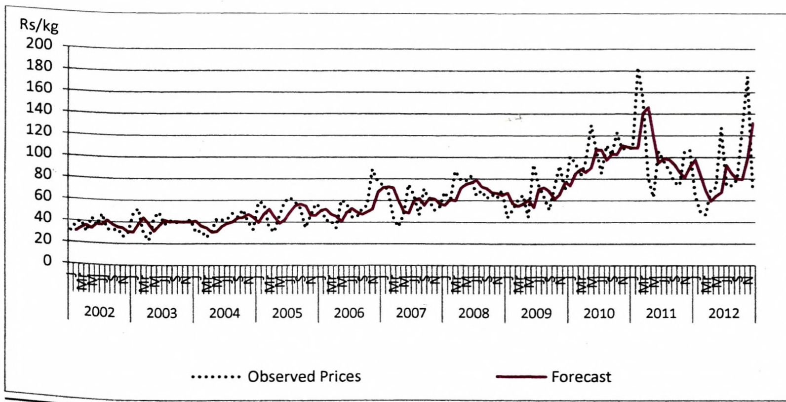
Figure 5.4: Single Exponential Smoothing Method (at alpha level 0.105) - Wholesale Prices of Tomato.
