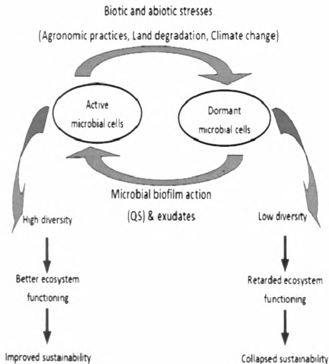
Figure 1. The interchange of dormant and active stages of microbes in the soil seed bank. Transition of metabolically active cells into dormant cells is a response to biotic and abiotic stresses induced by the human and the environment. Developed biofilms switch dormant cells to become metabolically active cells, thus improving sustainability in agroecosystems through increased microbial diversity and ecosystem functioning (Seneviratne et al. , 2013).
