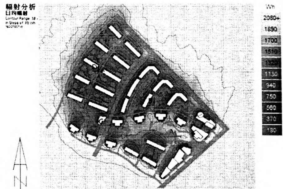
Fig.12: Average solar radiation throughout the day in winter
