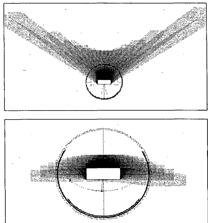
Fig.1: Greater cold days and the summer solstice continuous shadow figure of a same building (time range 7:00-15:30, time interval is 30min)
