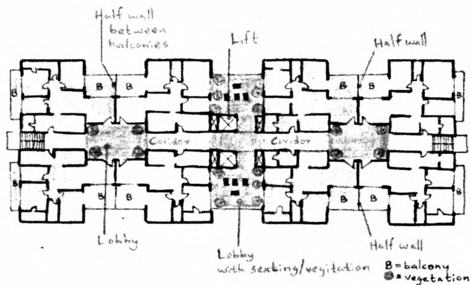
Fig 33 – Suggested layout in case 02 for enhancing SOC Source- Author
