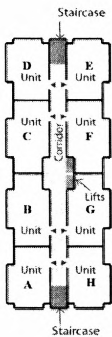
Fig 9- Type 1- Central court with two staircase elements at both ends Source- Author
