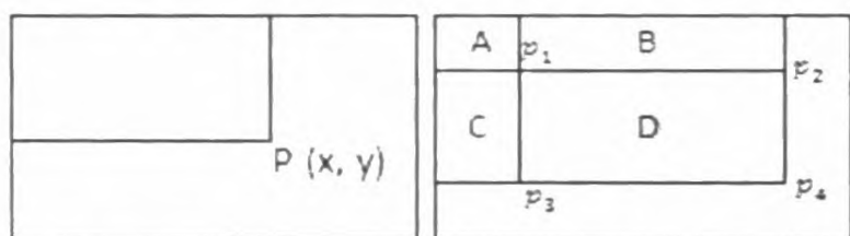
Figure 3: Integral image concept
