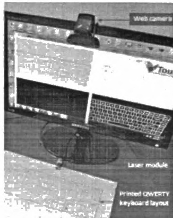
Figure 5: Hardware setup
