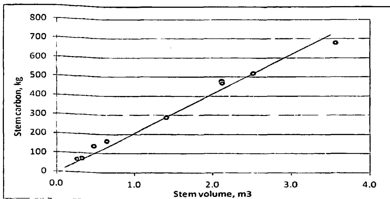
Figure 9: Average stem carbon values and the fitted line of equation 16.
