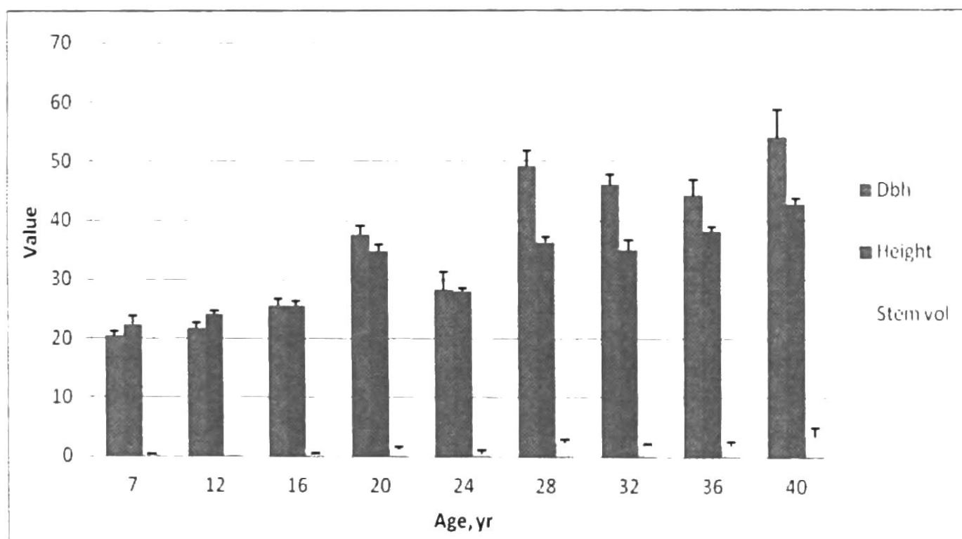
Figure 1: Variation of average dbh (cm), height (m) and volume (m 3 ) values with ( \pm SE).
