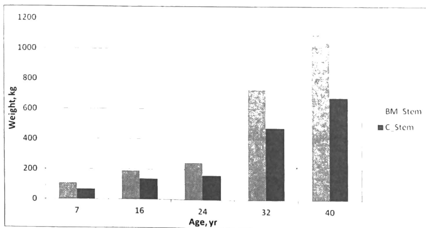
Figure 2: Variation of stem biomass and carbon values with the age.
