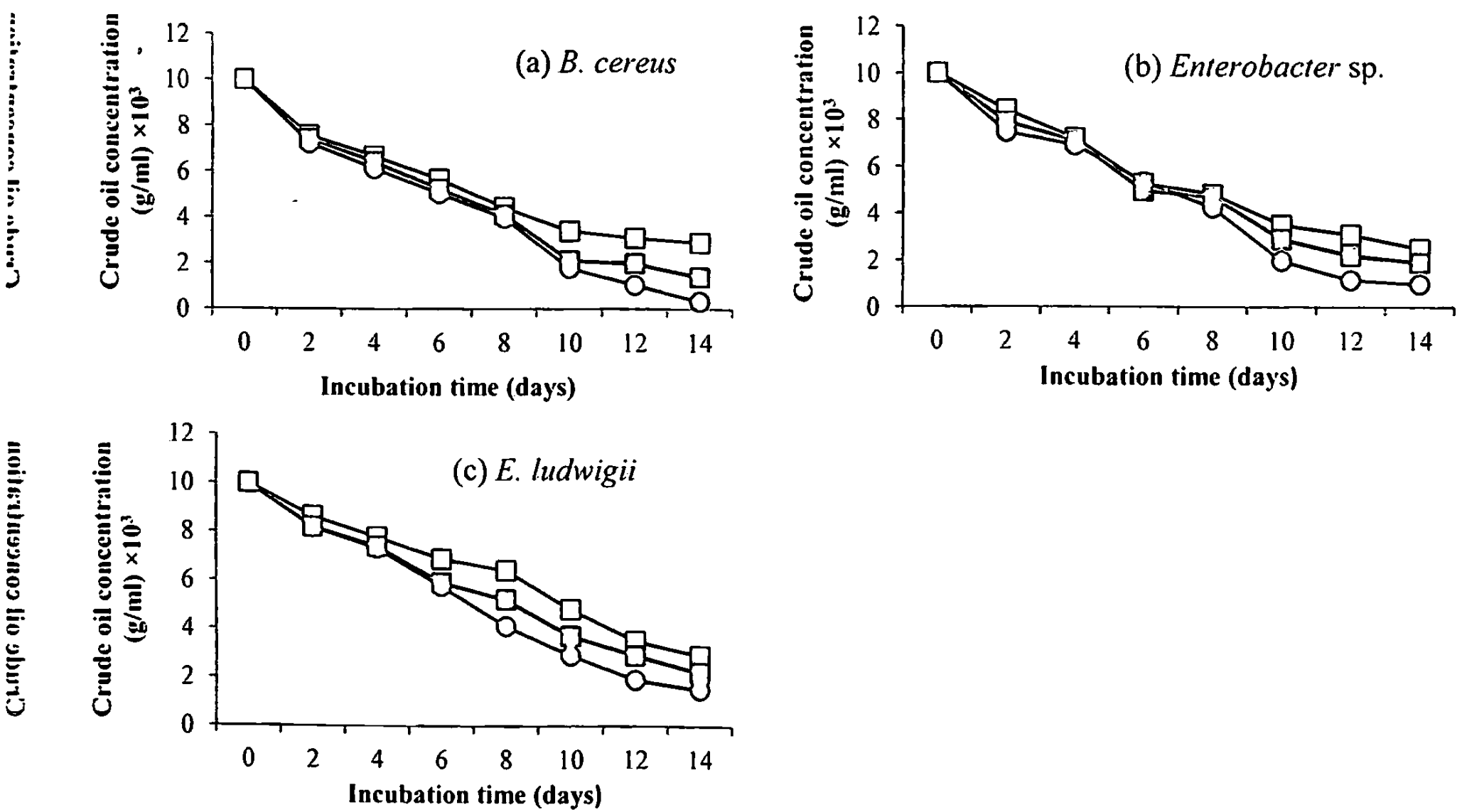
Figure 3: Degradation of crude oil (0.01 g/ml) by bacteria in the presence of nitrate.
