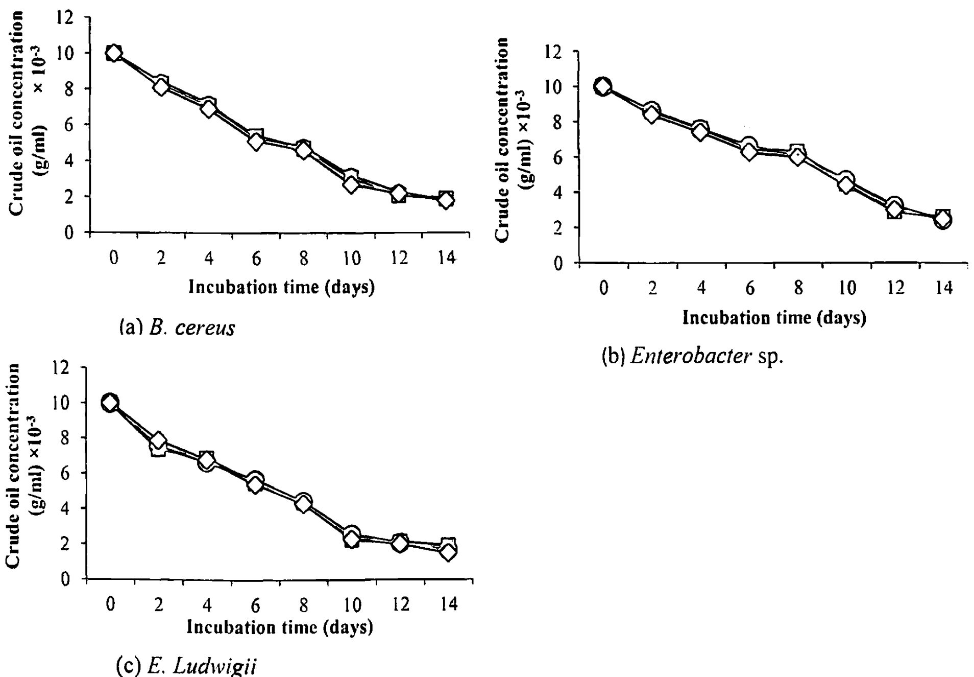
Figure 2: Degradation of crude oil (0.01 g/ml) by bacteria isolates with phosphate enrichment. (a) B. cereus (b) Enterobacter sp. (c) E. ludwigii ; 0.002 ppm (close square), control (close circle) and 0.05 ppm (open square).
