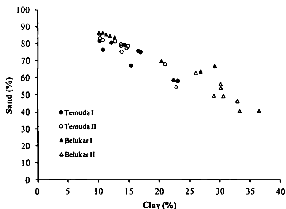
Figure 3: Relationship between sand and clay contents at the depth of 0-10 cm in the study sites. Temuda I ( y=-1.76x+100.37 , R^2=0.80 ), Temuda II ( y=-1.41x+98.13 , R^2=0.90 ), Belukar I ( y=-1.23x+98.93 , R^2=0.95 ), and Belukar II ( y=-1.47x+94.85 , R^2=0.63 ).
