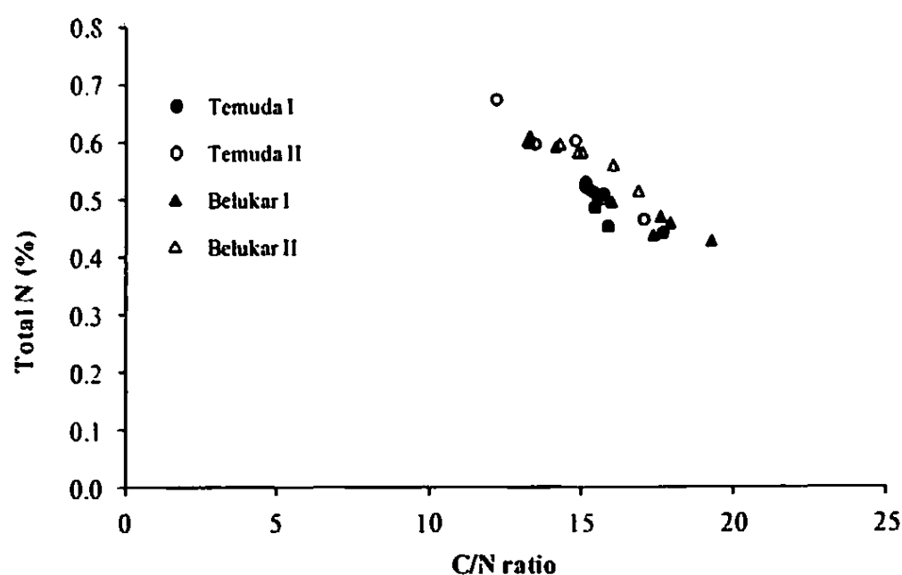
Figure 2: Relationship between total N and C/N ratio at the depth of 0-10 cm in the study sites. Temuda I ( y=-0.03x+0.98 , R^2=0.68 ), Temuda II ( y=-0.04x+1.20 , R^2=0.86 ), Belukar I ( y=-0.03x+0.91 , R^2=0.77 ), and Belukar II ( y=-0.03x+0.96 , R^2=0.74 ).
