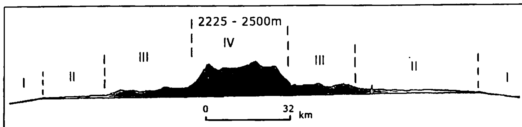
Figure 1: Diagrammatic section across Sri Lanka from west to east showing the four planated surfaces. I - first (submerged), II- second (Flat terrain to Undulating terrain, Rolling and Hilly Terrains, III - third (Dissected Rolling and Hilly: Steeply Dissected Rolling and Hilly Terrains, and IV - fourth (Mountainous and Rugged Central Highland)
