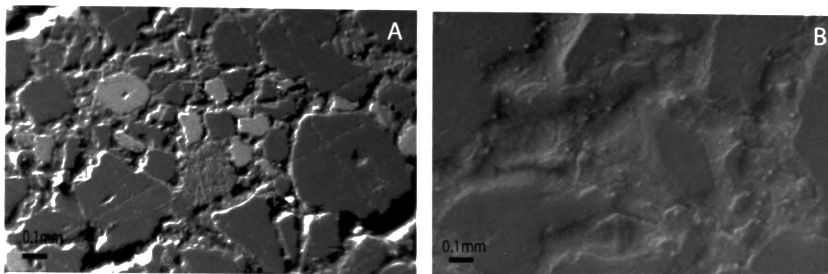
Fig. 4 SEM images of a tube burrow. A. Burrow has compacted fine to medium grains in a clayey matrix. B. Tiny pyrite octahedral crystals could be observed in the clayey matrix.
