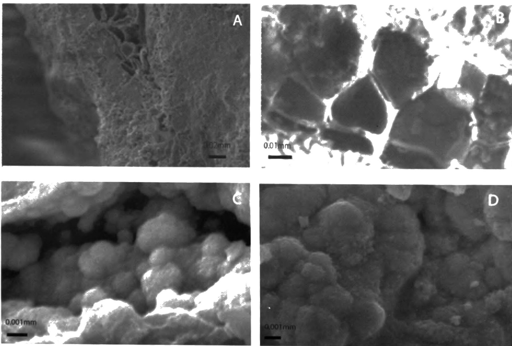
Fig. 6 SEM images of the internal wall lining of the tube. A. Sclerite shows honeycomb like structure. B. The innermost part of the inner wall has angular loose crystals probably chamosite or berthierine. C. and D Framboids of pyrite filled the honeycomb like structure
