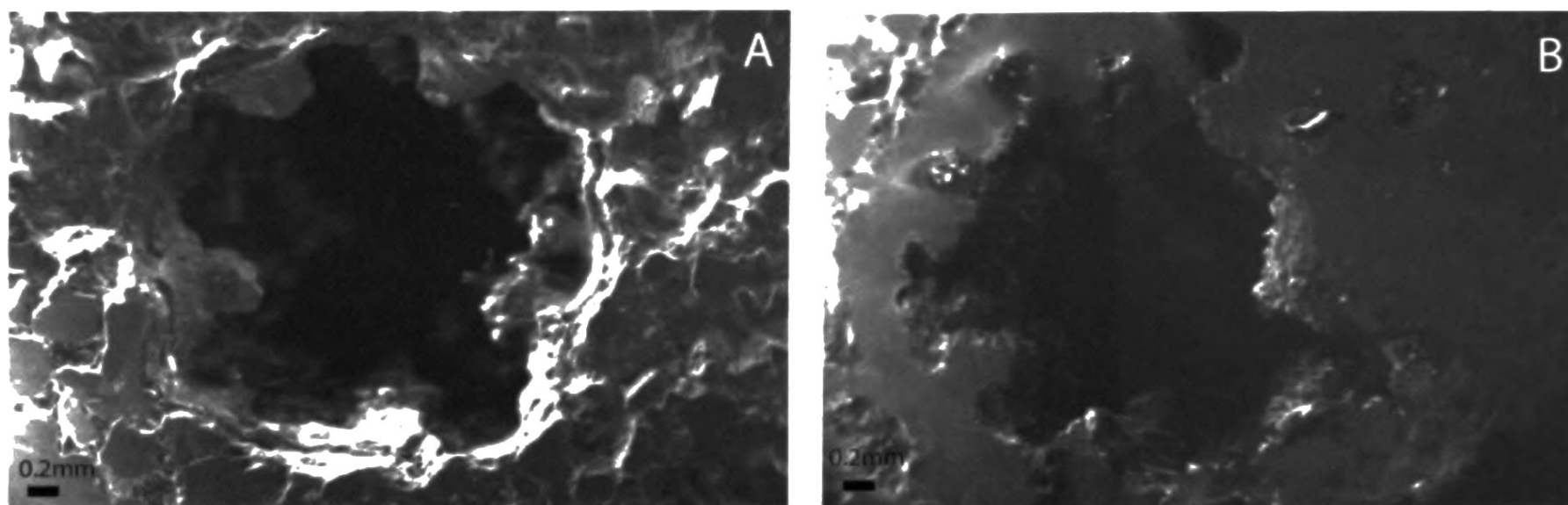
Fig. 5 SEM images of the irregular internal cross section of the tube burrows. A and B are two different sections.
