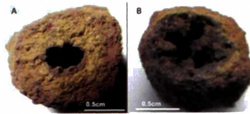
Fig. 3 Cross sections of the tube burrows. A and B are two selected specimens. Color rims around the center hole shows dark inner wall and reddish outer wall with yellow color low oxidized zone in between.
