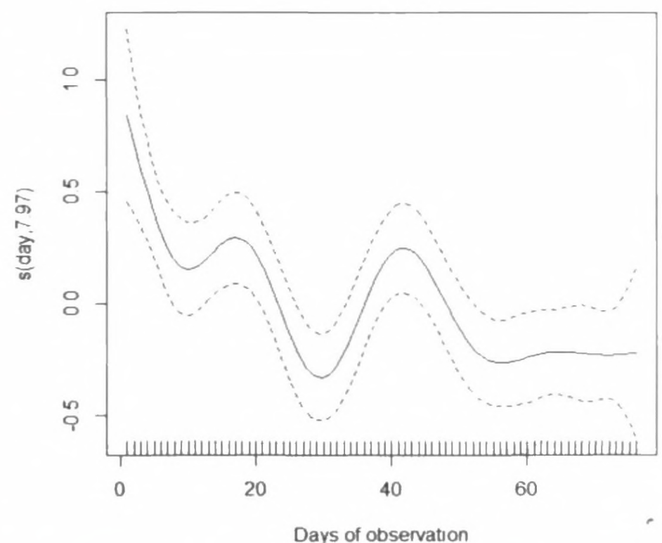
Figure 4. Non-parametric smoother through successive days of observations.
