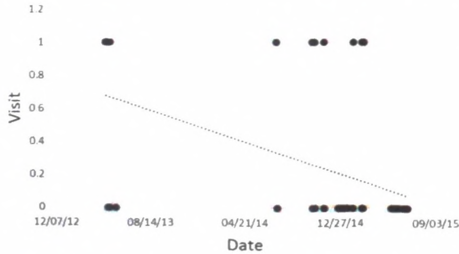
Figure 3. Linear regression line through observations from 20 th April 2013 to 23 rd June 2015.
