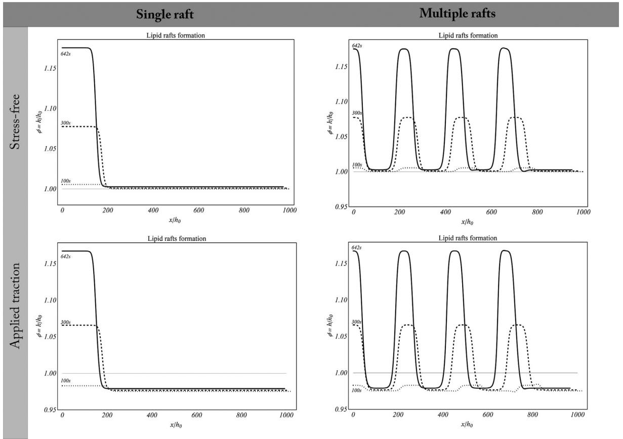
Fig. 6. Lipid raft formation in stress-free (upper row) and tensed (lower row) membranes. Both the case of a single raft and multiple raft are analysed, the membrane thickening following the activation of transmembrane proteins.
