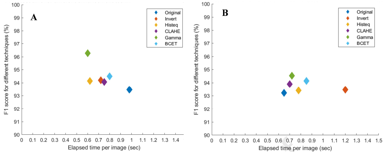
Figure 9. Comparison of F1 Score versus the elapsed time per image for the best performing network in each image enhancement technique for plain X-ray images (A) and segmented lung X-ray images (B).
