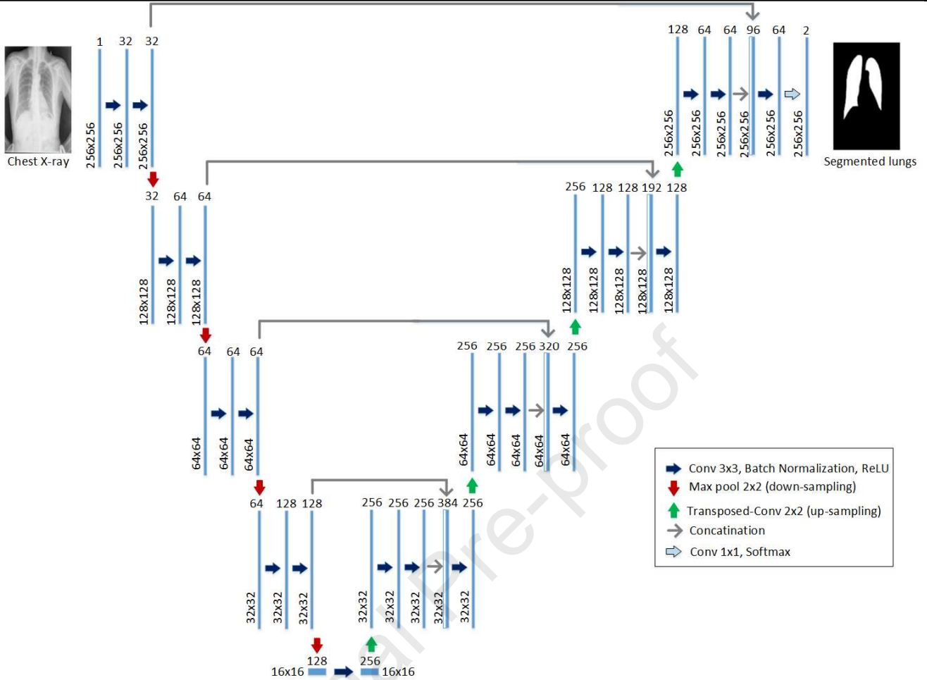
Figure 6: Modified U-Net model architecture proposed for lung segmentation.
