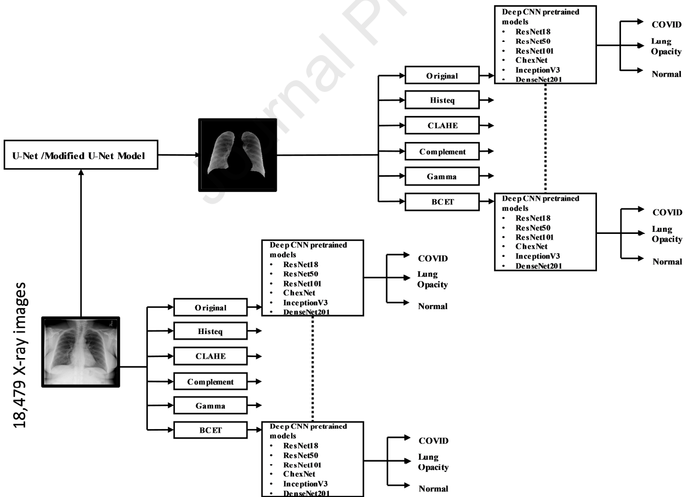
Figure 3: Block diagram of the system methodology.
