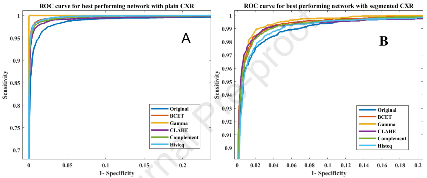
Figure 8. ROC curves for the best performing network in each image enhancement technique for plain CXR images (A) and segmented lung CXR images (B).
