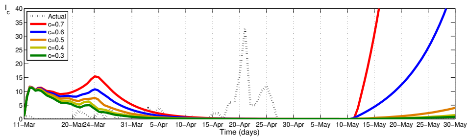
Fig. 3: Comparison of actual infected data and simulation results for different contact rate values in Colombo district
