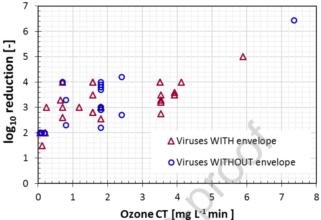
Figure 3: CT value vs \log_{10} virus reduction for surfaces disinfection. It shows those experiments from Table S2 in Supplementary Material (extended version), with a relative humidity higher than 65% and virus deposited in solid matrixes and moderate ozone exposure ( CT < 10 \text{ mg L}^{-1} \text{ min} ) (59 points from 10 publications).
