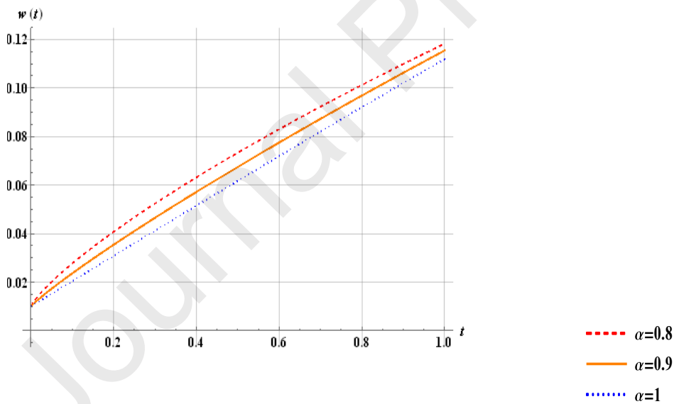
Fig.4 (f). Plots of w(t) vs. t with initial conditions x_0 = 0.6, y_0 = 0.25, z_0 = 0.20, u_0 = 0.05, v_0 = 0.02, w_0 = 0.01 and parameter values given in table when \alpha = 0.8, 0.9, 1 .
