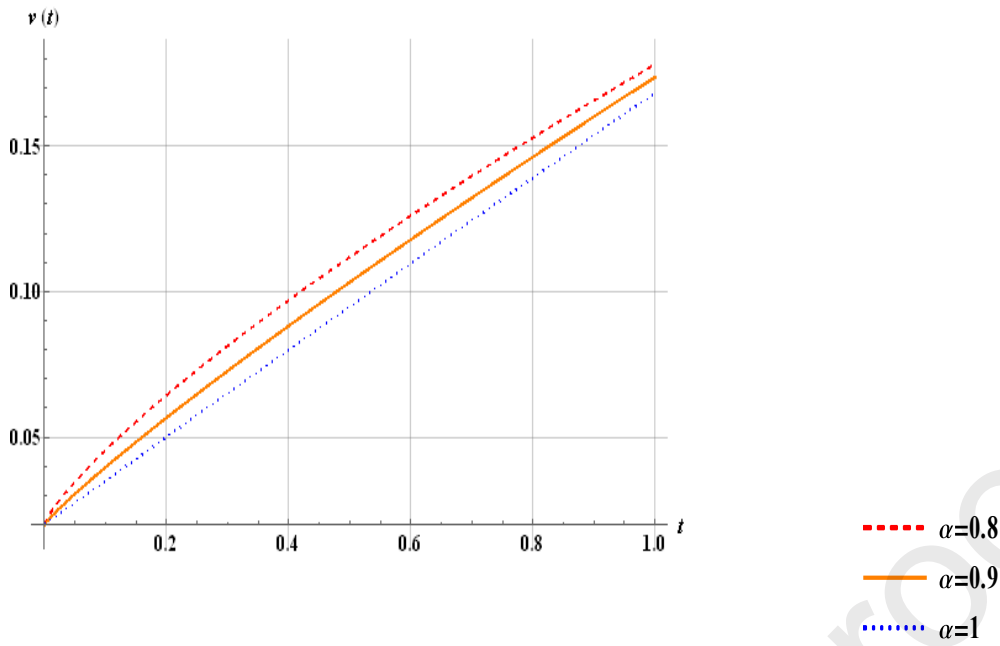
Fig.4 (e). Plots of v(t) vs. t with initial conditions x_0 = 0.6, y_0 = 0.25, z_0 = 0.20, u_0 = 0.05, v_0 = 0.02, w_0 = 0.01 and parameter values given in table when \alpha = 0.8, 0.9, 1 .
