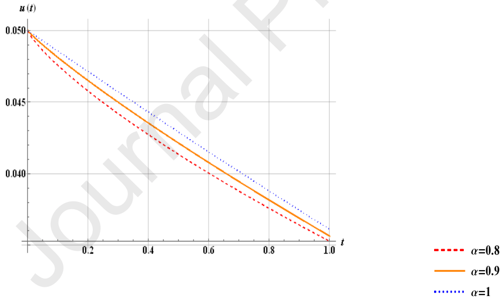
Fig.4 (d). Plots of u(t) vs. t with initial conditions x_0 = 0.6, y_0 = 0.25, z_0 = 0.20, u_0 = 0.05, v_0 = 0.02, w_0 = 0.01 and parameter values given in table for \alpha = 0.8, 0.9, 1 .
