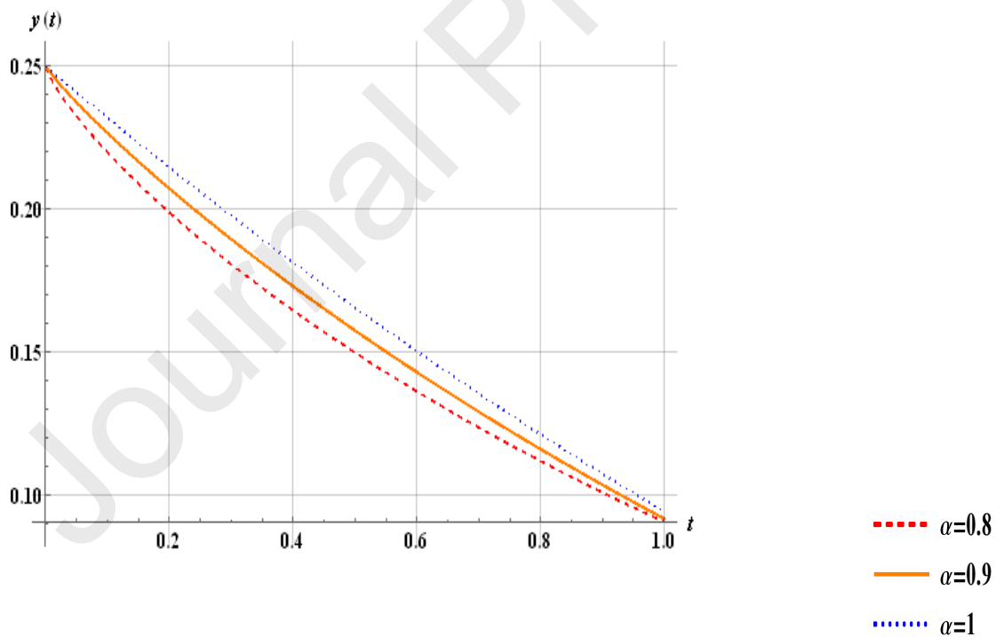
Fig.4 (b). Plots of y(t) vs. t with initial conditions x_0 = 0.6, y_0 = 0.25, z_0 = 0.20, u_0 = 0.05, v_0 = 0.02, w_0 = 0.01 and parameter values given in table when \alpha = 0.8, 0.9, 1 .
