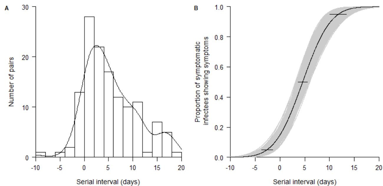
Fig. 2. A) Distribution of the observed serial interval of 131 pairs with confirmed close contact; B) Cumulative distribution function of the serial interval of COVID-19 under the Weibull distribution model. Horizontal bars represent the 95% CIs of the 2.5th, 50th, and 97.5th percentiles of the serial interval distribution.
