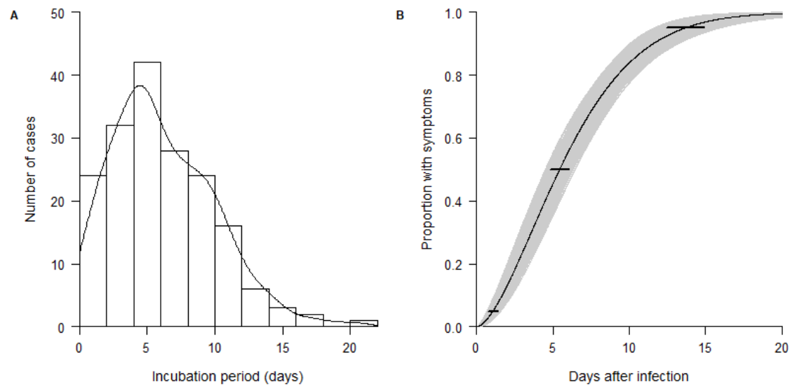
Fig. 1. A) Distribution of the observed incubation period of 178 COVID-19 cases; B) Cumulative distribution function of the incubation period of COVID-19 under the Weibull distribution model. Horizontal bars represent the 95% CIs of the 2.5th, 50th, and 97.5th percentiles of the incubation period distribution.
