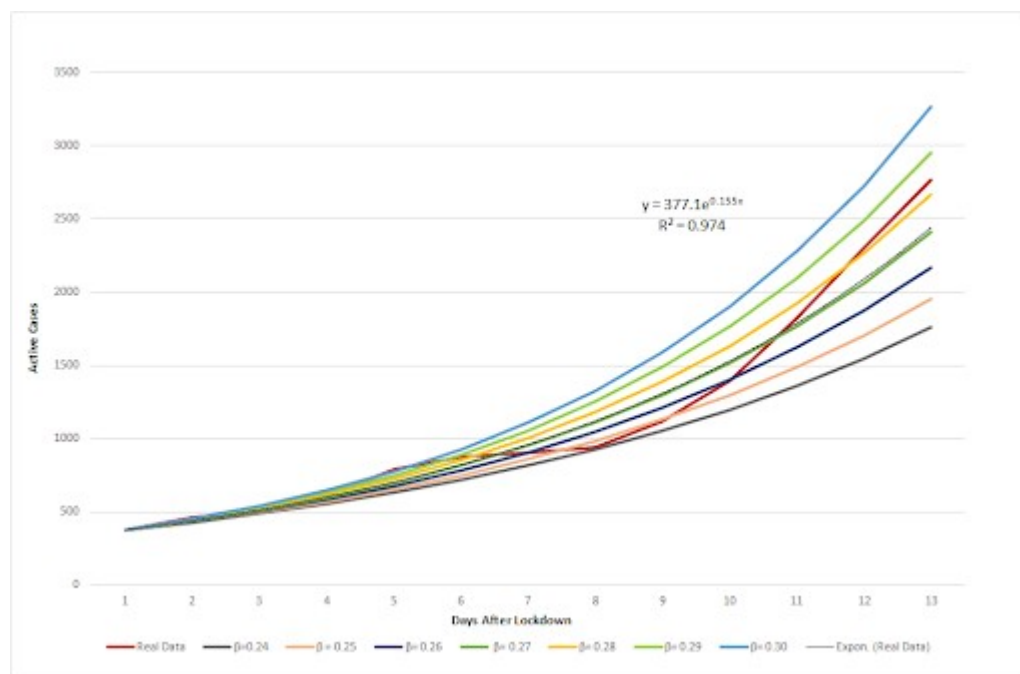
Appendix Table: Output of the model run by varying \beta
